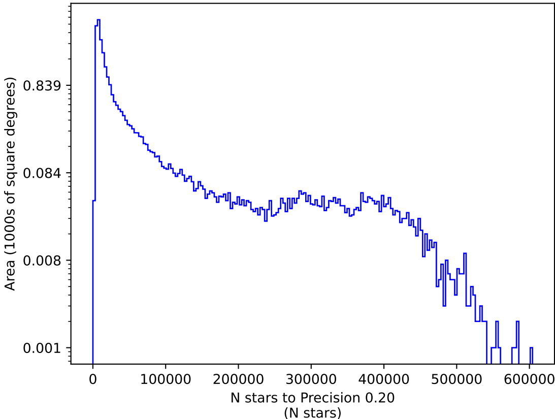
ddf_acor_sf15_lsf20_lsr10_v3.4_10yrs g: N stars to Precision 0.20
