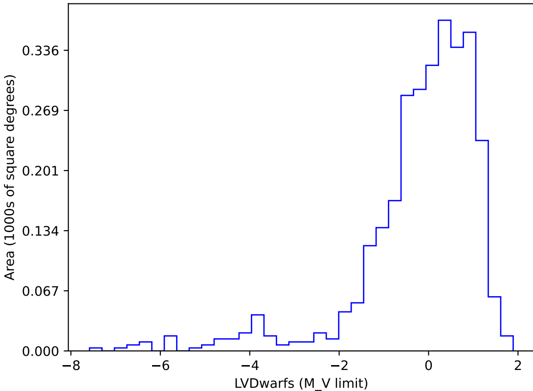
ddf_acor_sf15_lsf20_lsr10_v3.4_10yrs gi SCP: LVDwarfs
