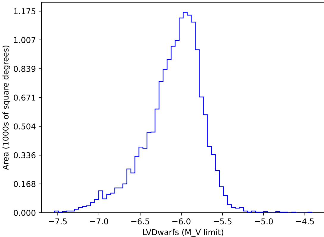
ddf_acor_sf15_lsf20_lsr10_v3.4_10yrs gi: LVDwarfs
