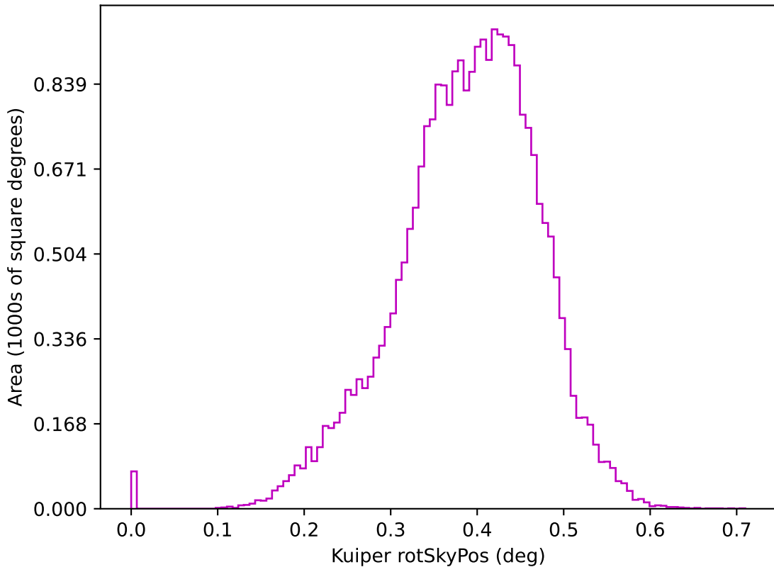
ddf_acor_sf15_lsf20_lsr10_v3.4_10yrs z: Kuiper rotSkyPos
