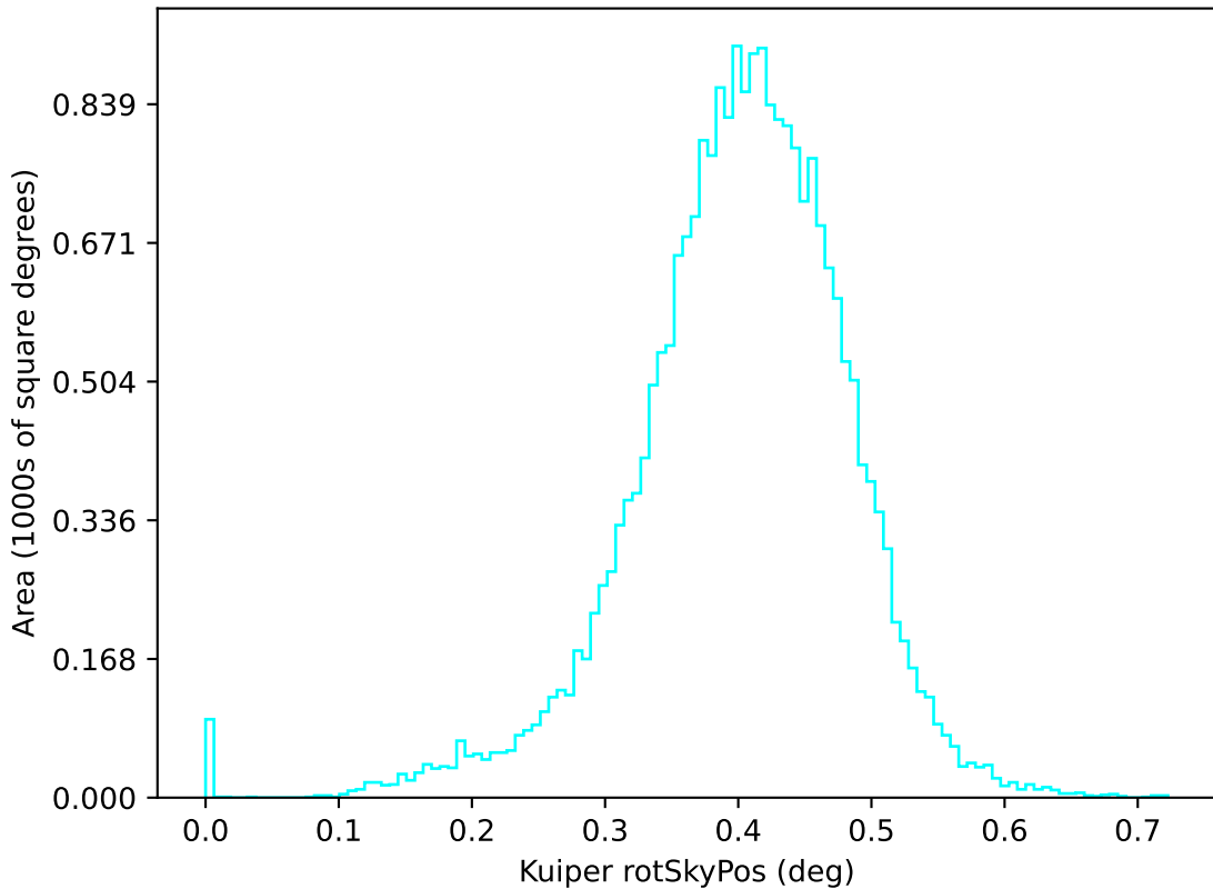
ddf_acor_sf15_lsf20_lsr10_v3.4_10yrs u: Kuiper rotSkyPos
