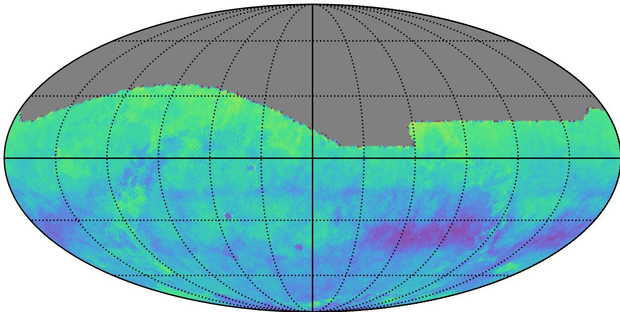
ddf_acor_sf15_lsf20_lsr10_v3.4_10yrs r: Kuiper rotSkyPos
