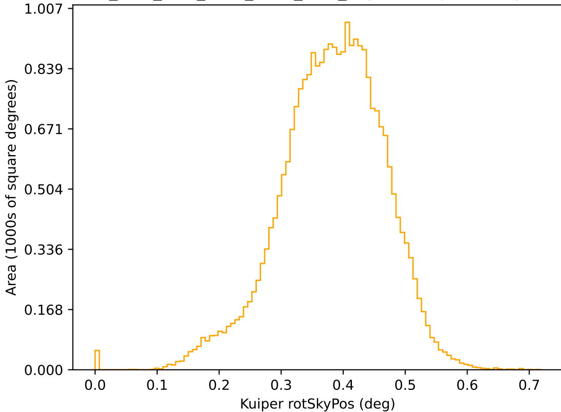
ddf_acor_sf15_lsf20_lsr10_v3.4_10yrs r: Kuiper rotSkyPos
