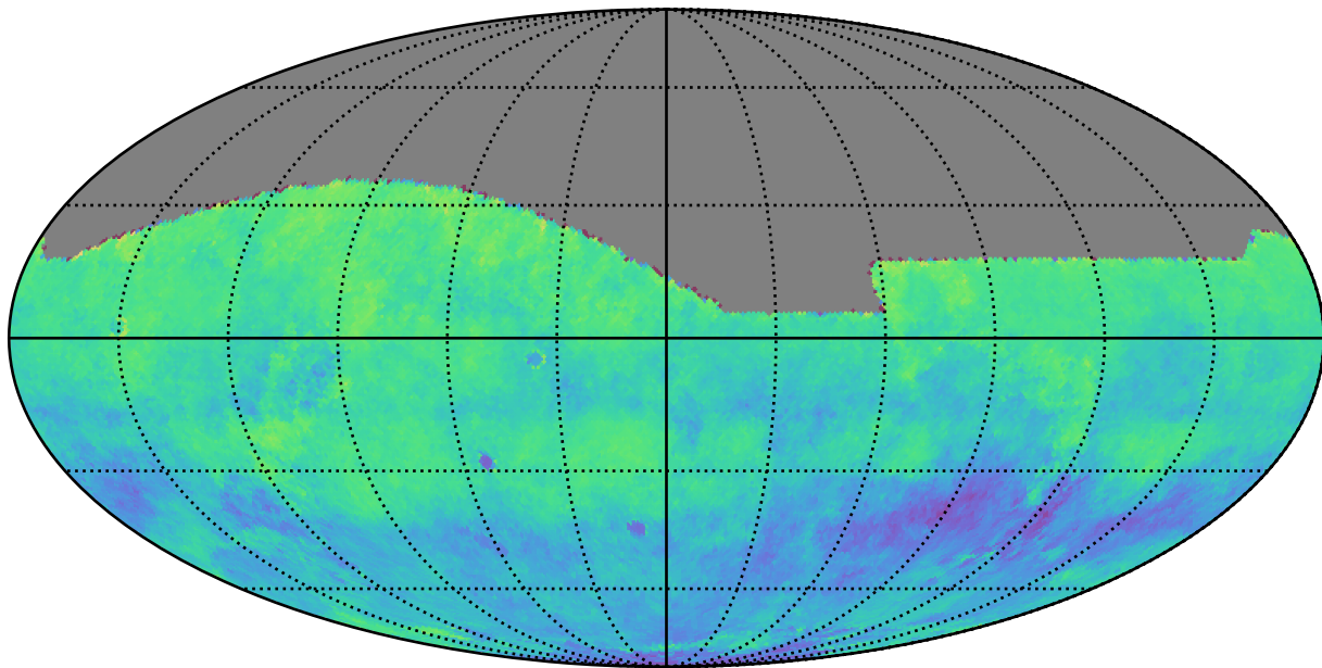
ddf_acor_sf15_lsf20_lsr10_v3.4_10yrs i: Kuiper rotSkyPos
