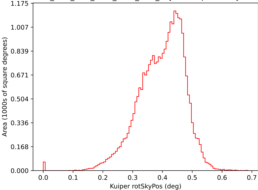
ddf_acor_sf15_lsf20_lsr10_v3.4_10yrs i: Kuiper rotSkyPos
