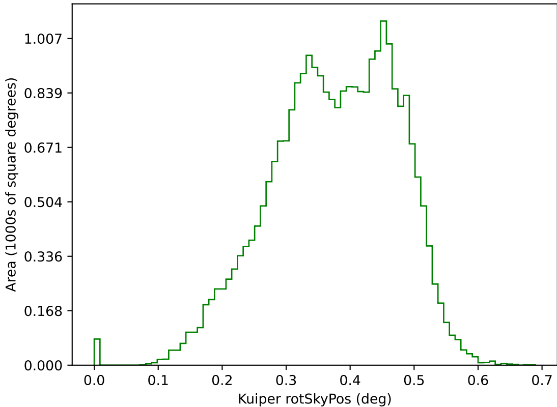
ddf_acor_sf15_lsf20_lsr10_v3.4_10yrs g: Kuiper rotSkyPos
