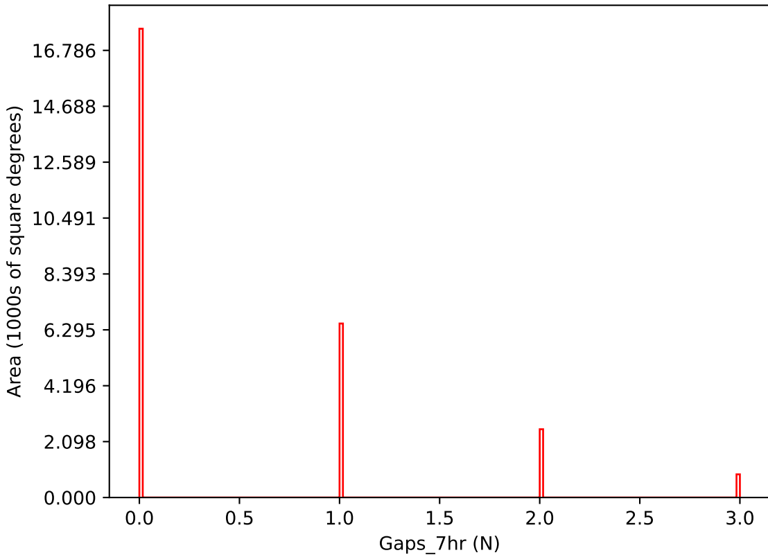
ddf_acor_sf15_lsf20_lsr10_v3.4_10yrs i band: Gaps_7hr
