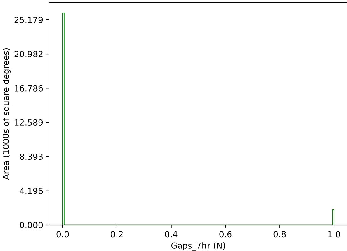
ddf_acor_sf15_lsf20_lsr10_v3.4_10yrs g band: Gaps_7hr
