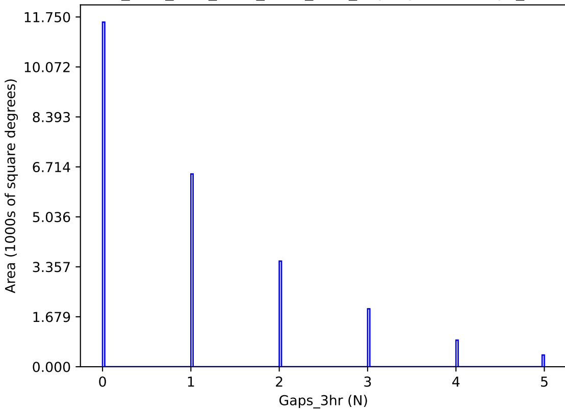
ddf_acor_sf15_ls20_lsr10_v3.4_10yrs y band: Gaps_3hr
