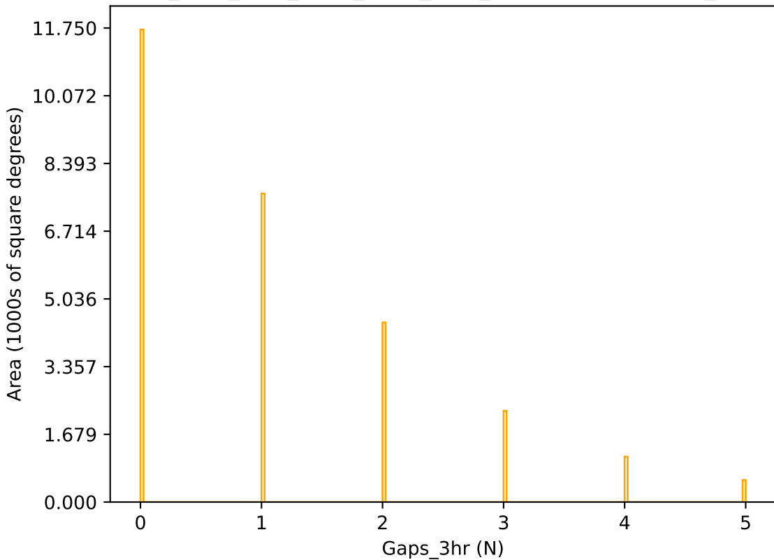
ddf_acor_sf15_lsf20_lsr10_v3.4_10yrs r band: Gaps_3hr
