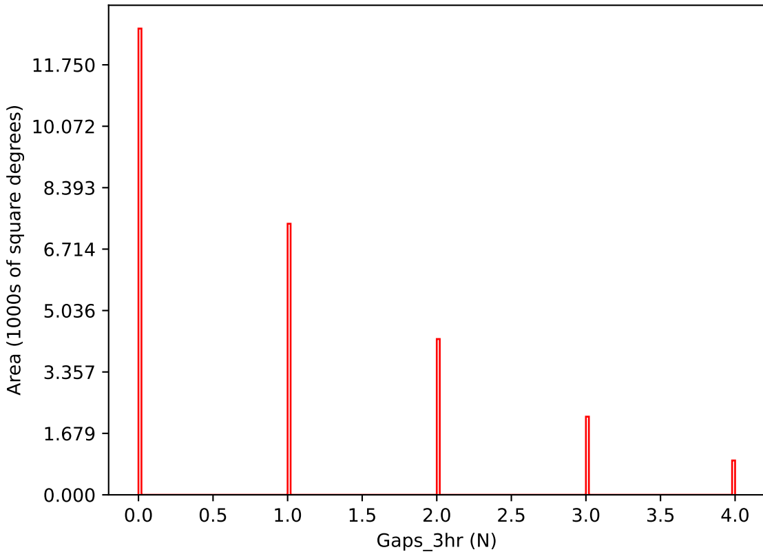
ddf_acor_sf15_lsf20_lsr10_v3.4_10yrs i band: Gaps_3hr
