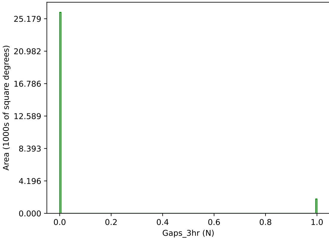
ddf_acor_sf15_lsf20_lsr10_v3.4_10yrs g band: Gaps_3hr
