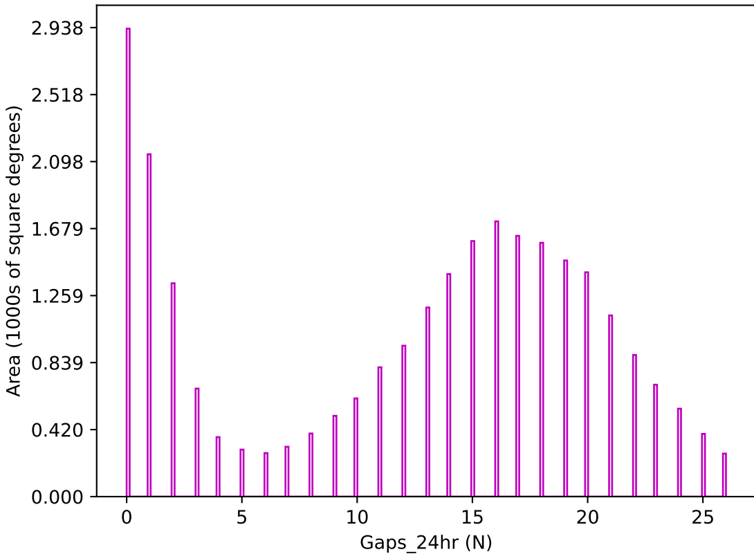
ddf_acor_sf15_ls20_lsr10_v3.4_10yrs z band: Gaps_24hr
