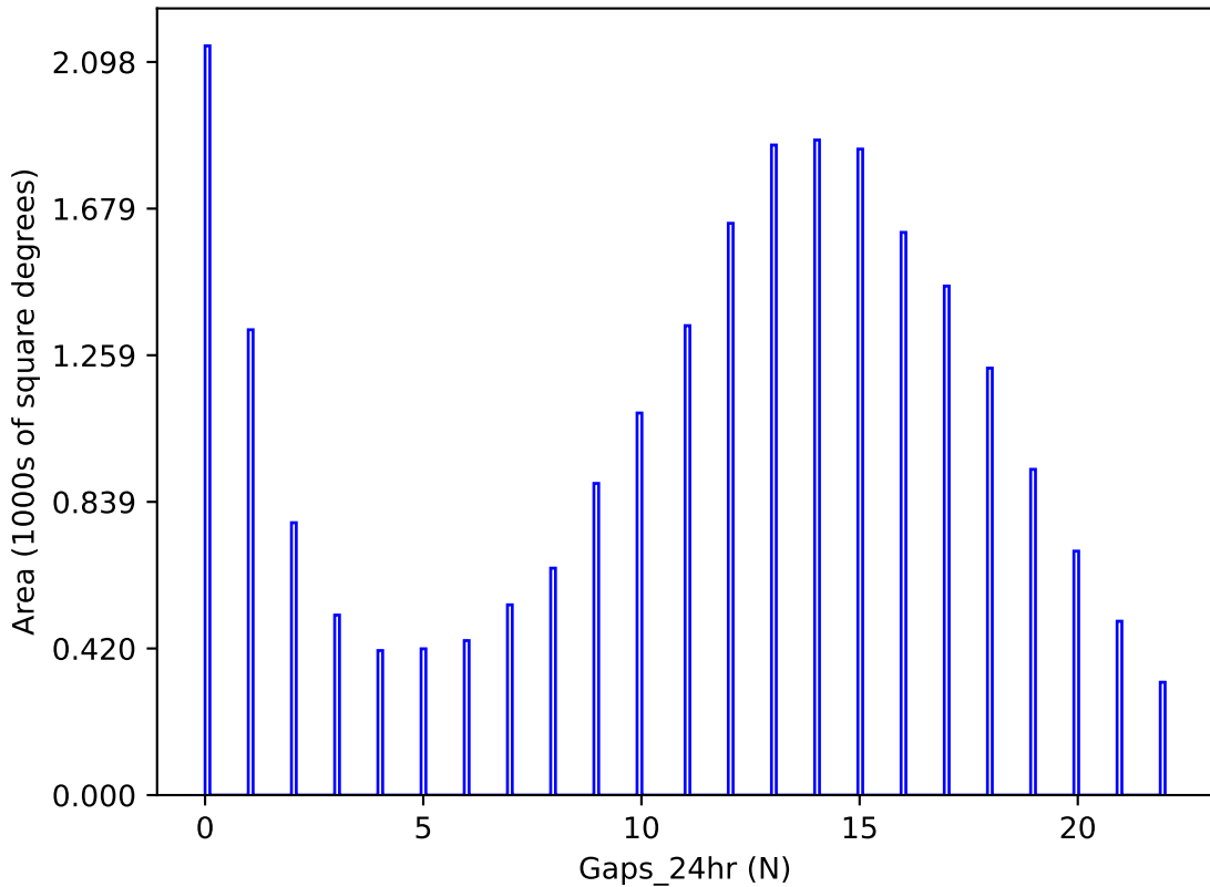
ddf_acor_sf15_lsf20_lsr10_v3.4_10yrs y band: Gaps_24hr
