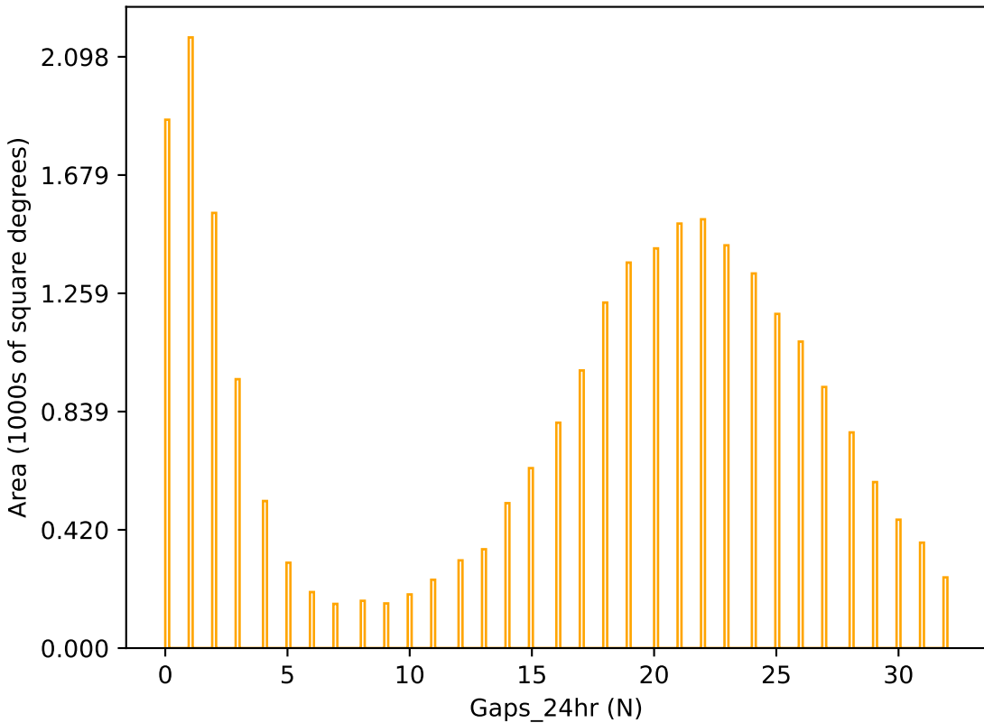
ddf_acor_sf15_lsf20_lsr10_v3.4_10yrs r band: Gaps_24hr
