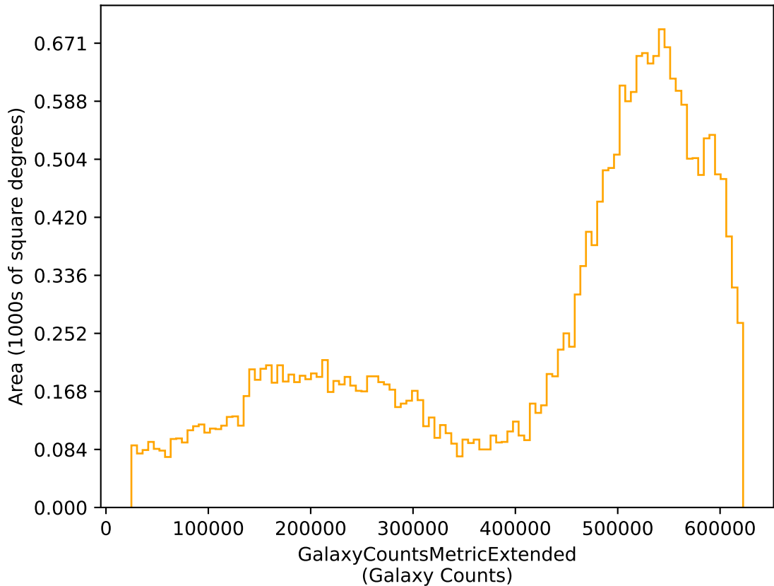
ddf_acor_sf15_lsf20_lsr10_v3.4_10yrs r: GalaxyCountsMetricExtended
