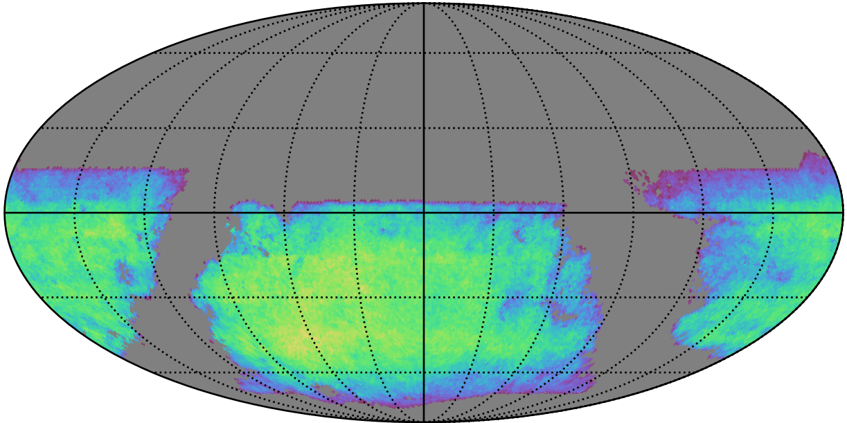
ddf_acor_sf15_lsf20_lsr10_v3.4_10yrs i band non-DD year 8: ExgalM5WithCuts
