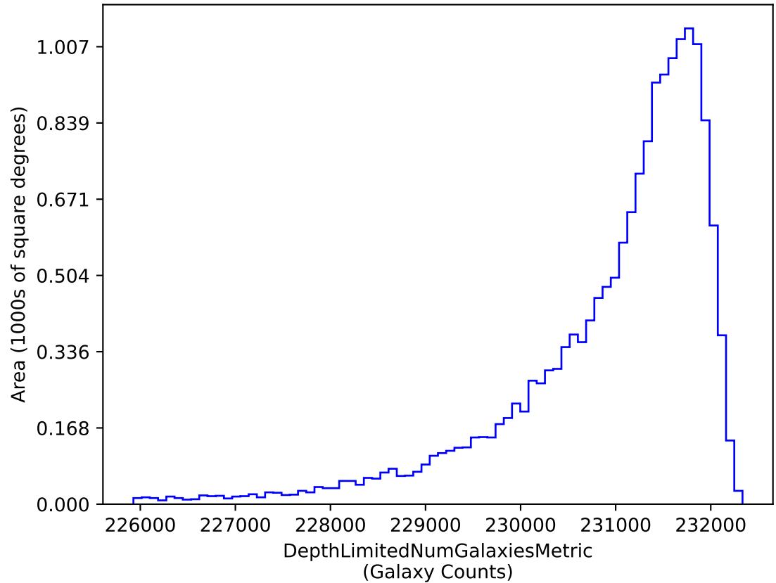
ddf_acor_sf15_lsf20_lsr10_v3.4_10yrs i band galaxies non-DD: DepthLimitedNumGalaxiesMetric
