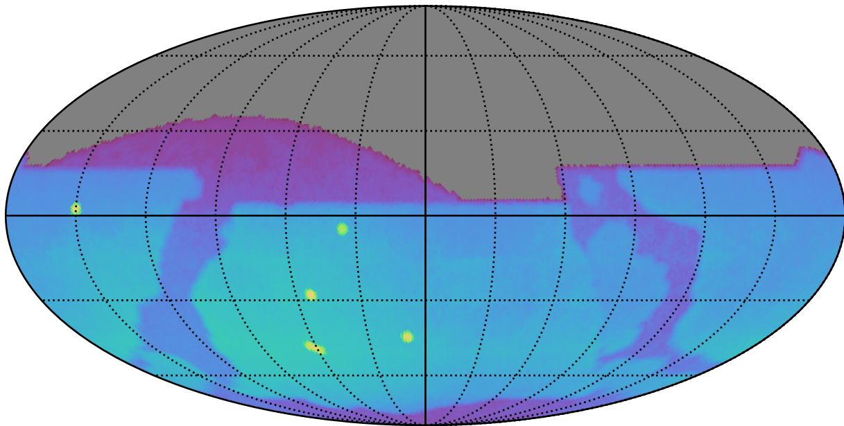
ddf_acor_sf15_lsf20_lsr10_v3.4_10yrs : Brown Dwarf, L7
