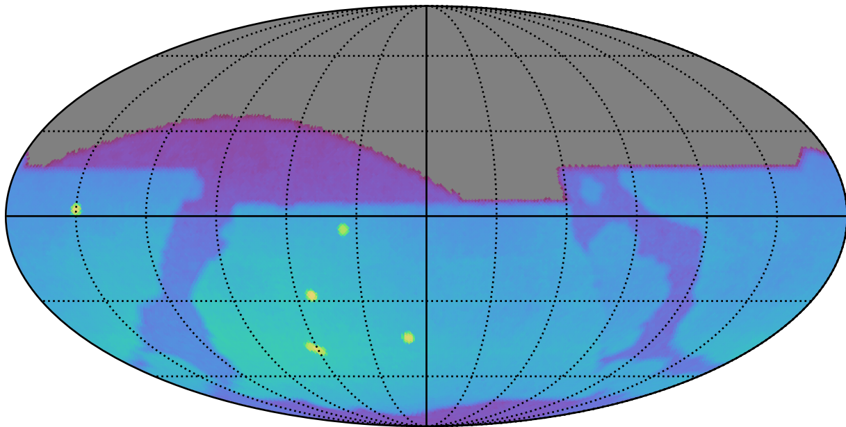
ddf_acor_sf15_lsf20_lsr10_v3.4_10yrs : Brown Dwarf, L4
