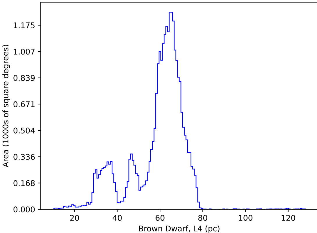
ddf_acor_sf15_lsf20_lsr10_v3.4_10yrs : Brown Dwarf, L4
