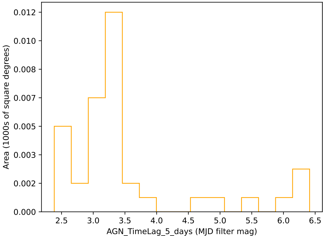
ddf_acor_sf15_lsf20_lsr10_v3.4_10yrs r band: AGN_TimeLag_5_days
