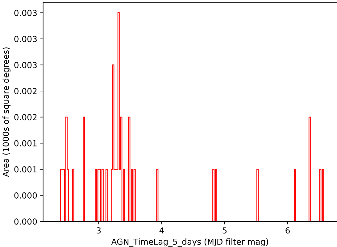
ddf_acor_sf15_lsf20_lsr10_v3.4_10yrs i band: AGN_TimeLag_5_days
