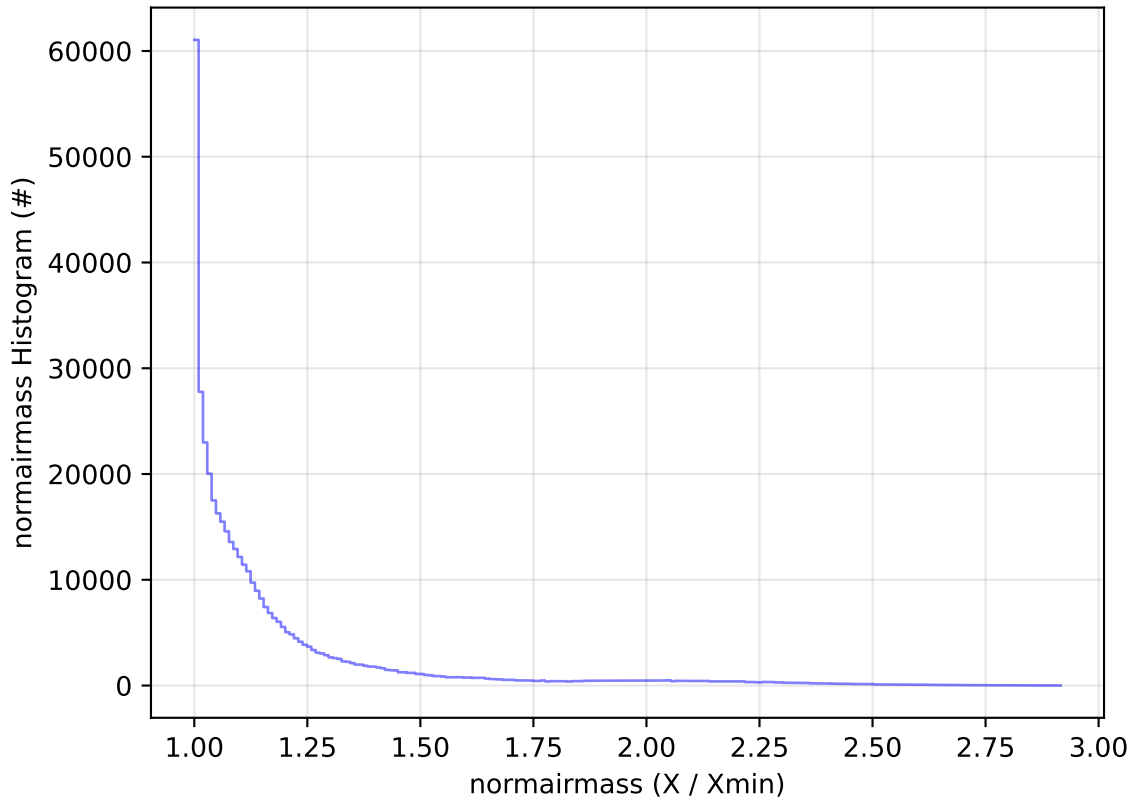
ddf_acor_sf15_lsf20_lsr10_v3.4_10yrs All sky z band: normairmass Histogram
