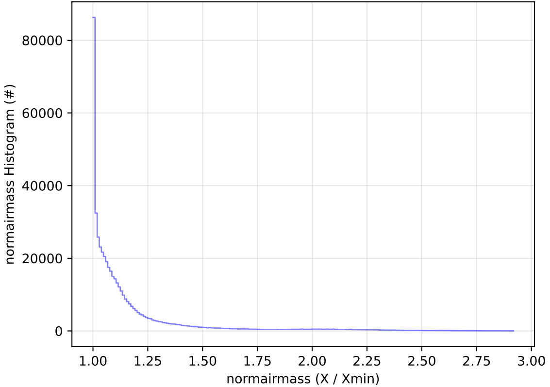
ddf_acor_sf15_lsf20_lsr10_v3.4_10yrs All sky i band: normairmass Histogram
