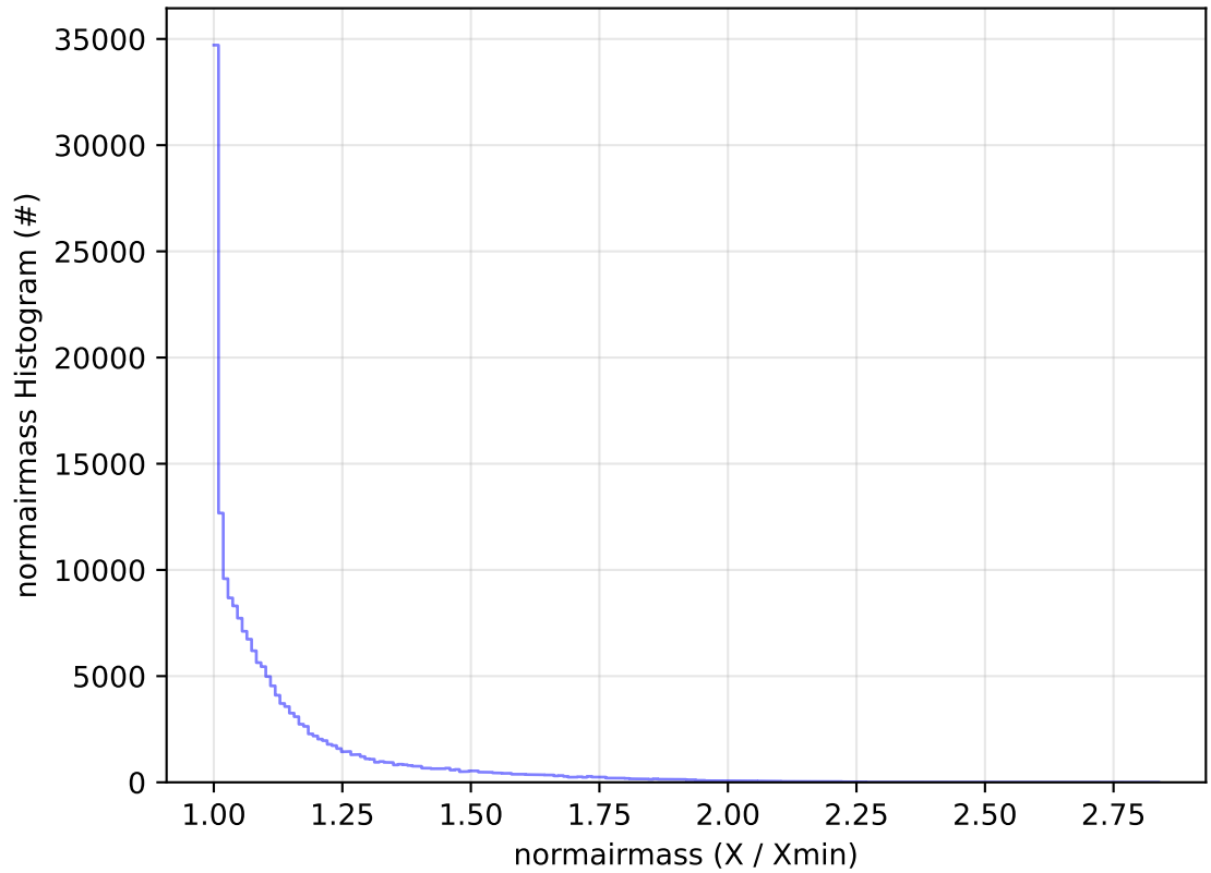
ddf_acor_sf15_lsf20_lsr10_v3.4_10yrs All sky g band: normairmass Histogram
