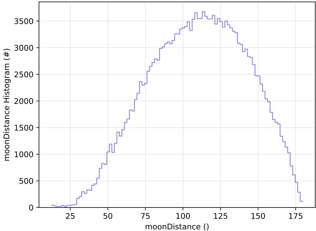
ddf_acor_sf15_lsf20_lsr10_v3.4_10yrs WFD g band: moonDistance Histogram
