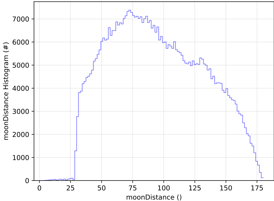
ddf_acor_sf15_lsf20_lsr10_v3.4_10yrs All sky i band: moonDistance Histogram
