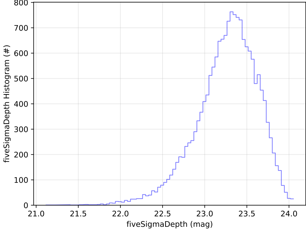
ddf_acor_sf15_lsf20_lsr10_v3.4_10yrs Yr 1 u band: fiveSigmaDepth Histogram
