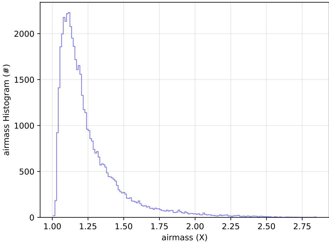
ddf_acor_sf15_ls20_lsr10_v3.4_10yrs Yr 1 y band: airmass Histogram
