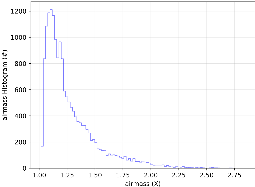
ddf_acor_sf15_lsf20_lsr10_v3.4_10yrs Yr 1 u band: airmass Histogram
