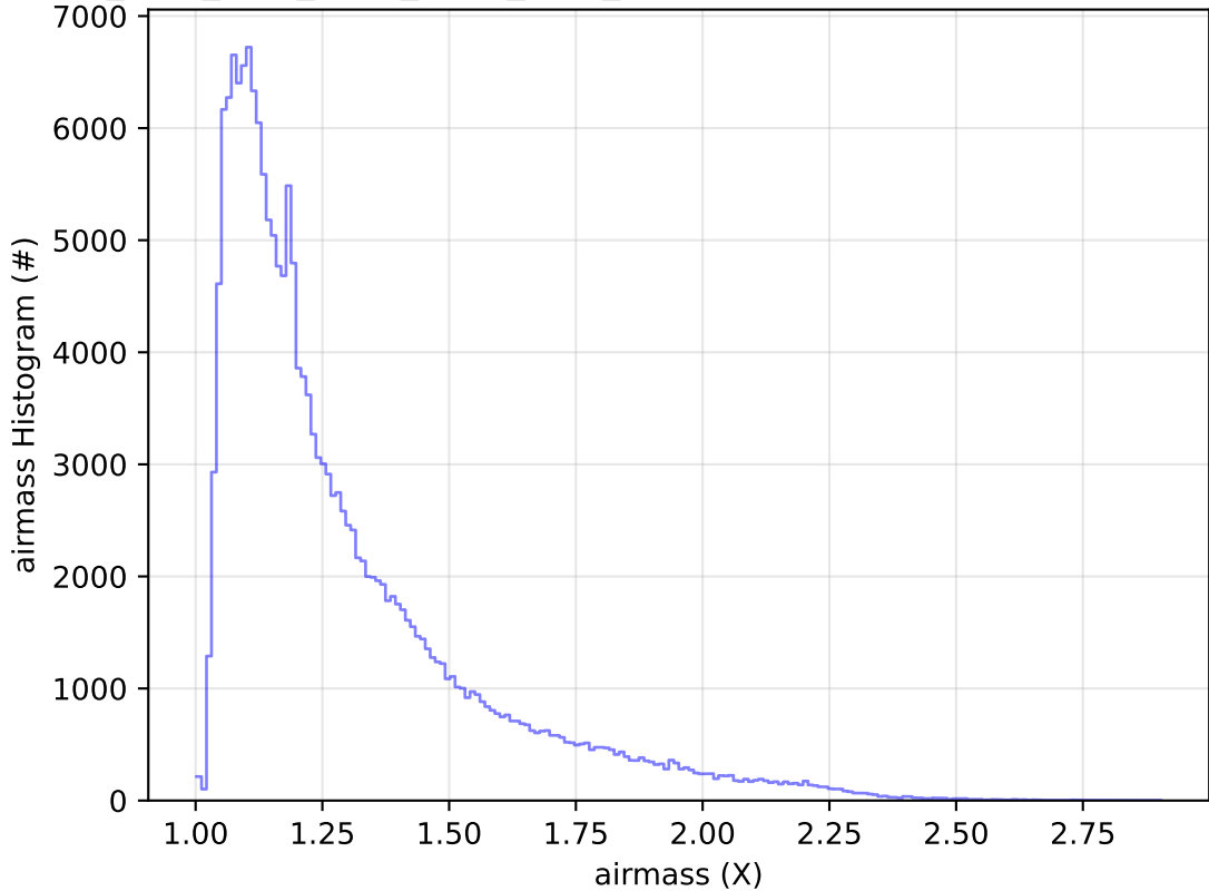
ddf_acor_sf15_lsf20_lsr10_v3.4_10yrs WFD g band: airmass Histogram
