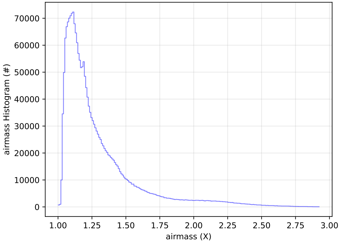
ddf_acor_sf15_lsf20_lsr10_v3.4_10yrs All sky all bands: airmass Histogram
