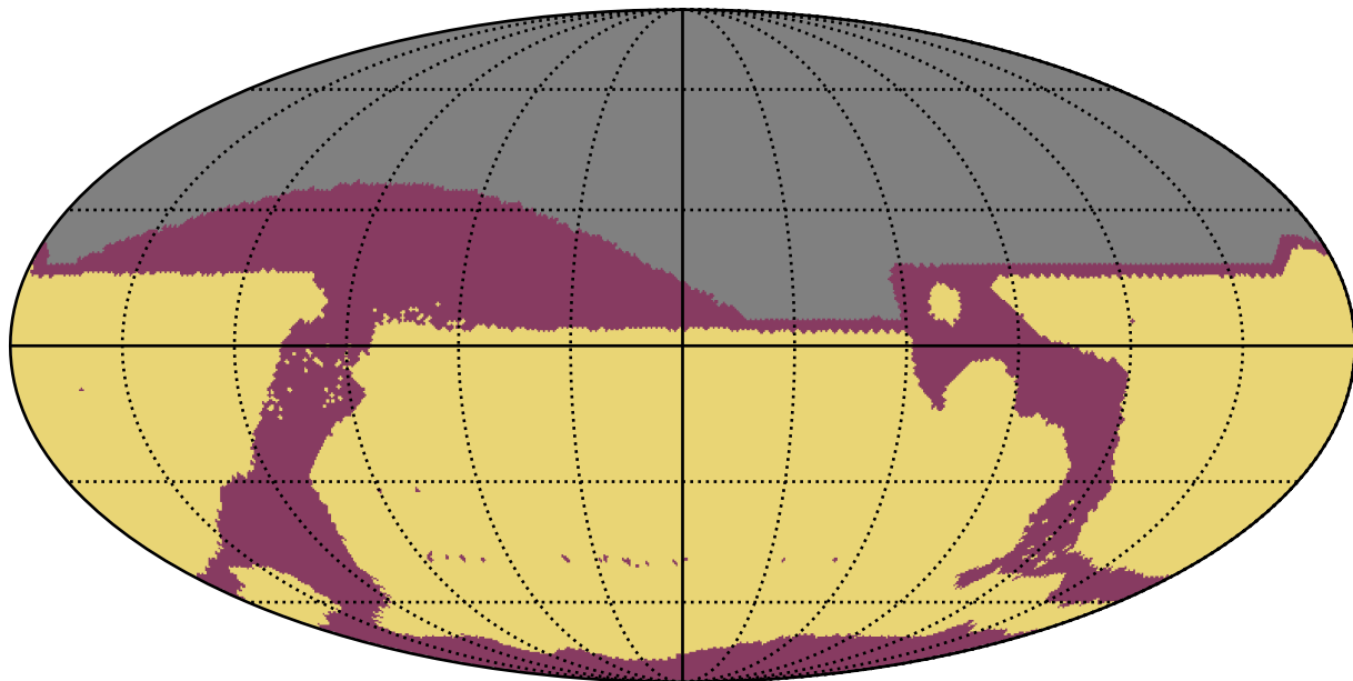
ddf_acor_sf15_lsf20_lsr10_v3.4_10yrs All sky: RapidRevisits
