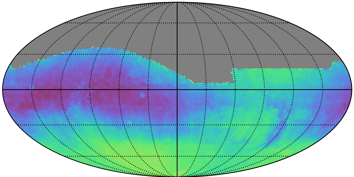
ddf_acor_sf15_lsf20_lsr10_v3.4_10yrs All sky: Parallax-DCR degeneracy @ 22.4
