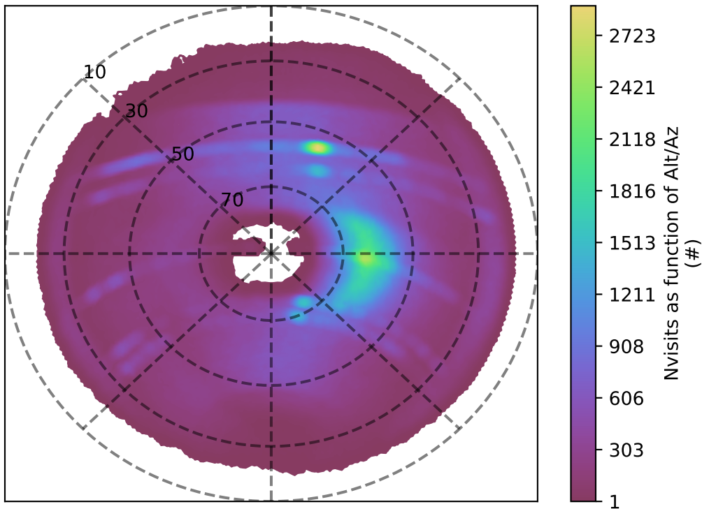
ddf_acor_sf15_lsf20_lsr10_v3.4_10yrs z band: Nvisits as function of Alt/Az
