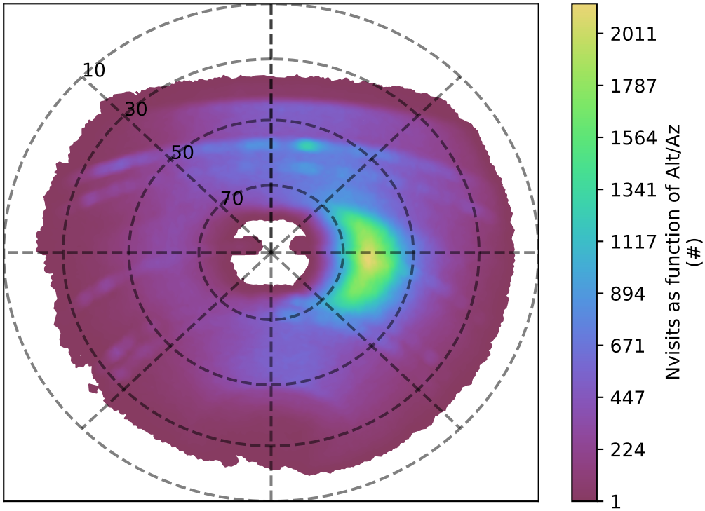
ddf_acor_sf15_lsf20_lsr10_v3.4_10yrs y band: Nvisits as function of Alt/Az
