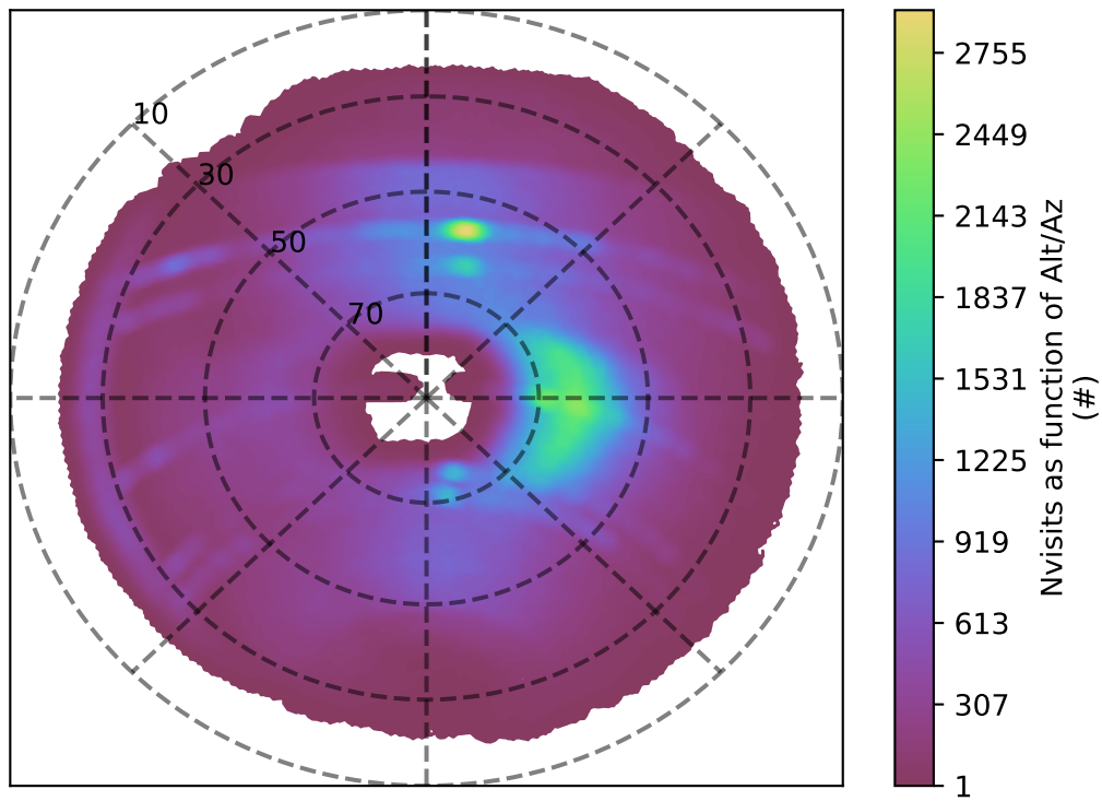
ddf_acor_sf15_lsf20_lsr10_v3.4_10yrs r band: Nvisits as function of Alt/Az
