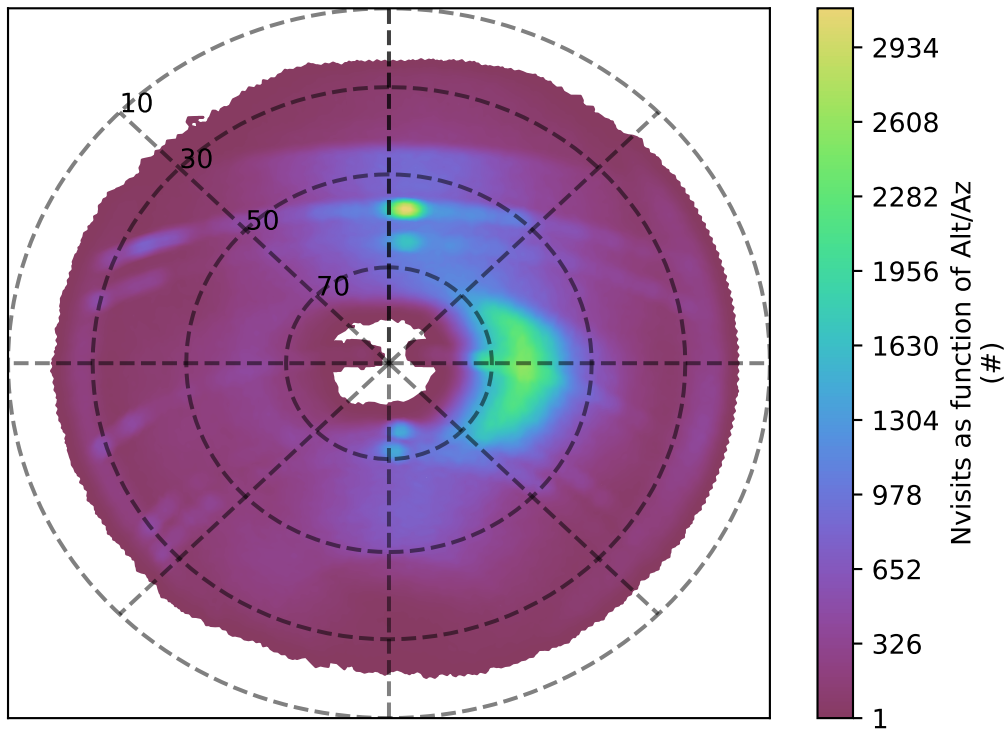
ddf_acor_sf15_lsf20_lsr10_v3.4_10yrs i band: Nvisits as function of Alt/Az
