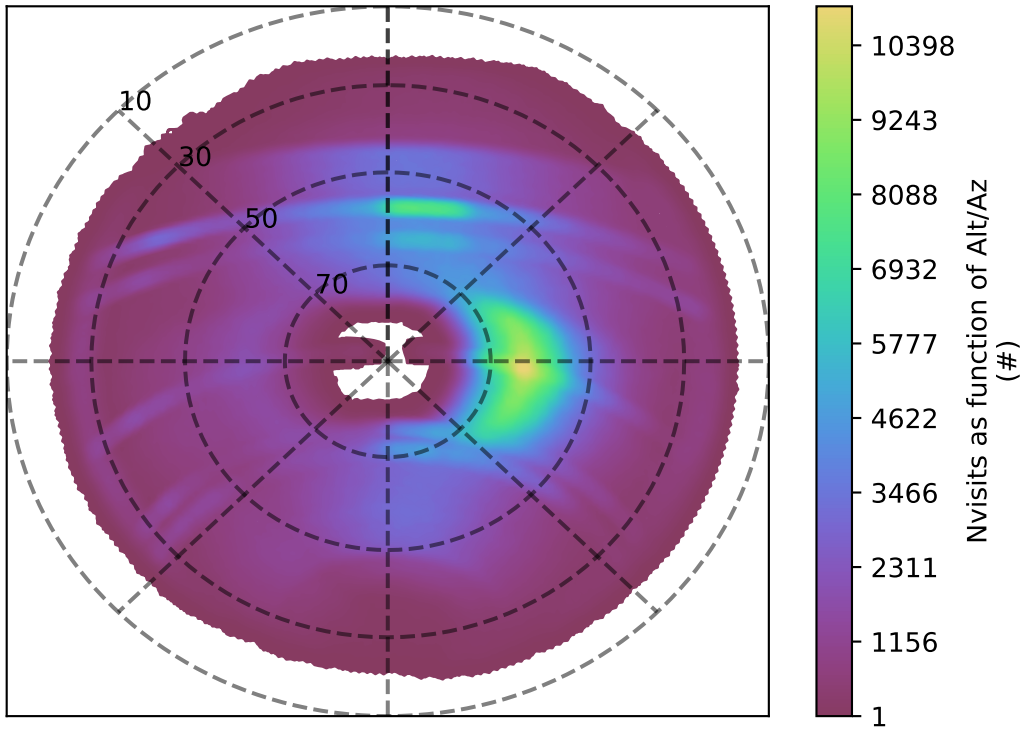
ddf_acor_sf15_lsf20_lsr10_v3.4_10yrs all bands: Nvisits as function of Alt/Az
