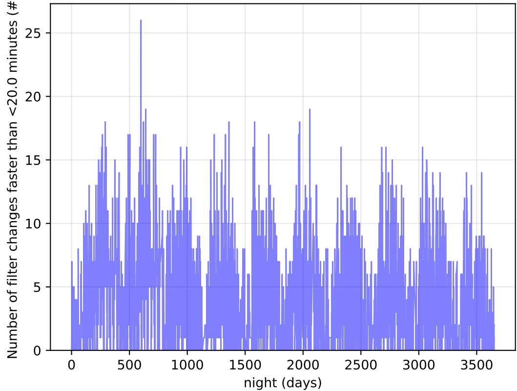
ddf_acor_sf15_Isf20_Isr10_v3.4_10yrs Per Night: Number of filter changes faster than <20.0 minutes
