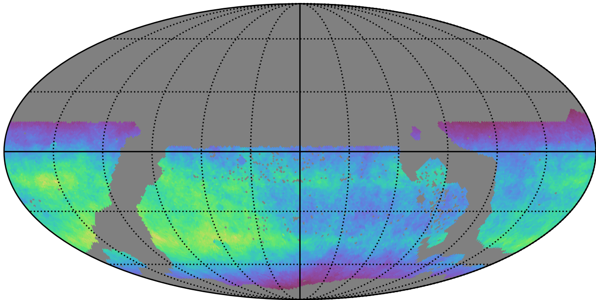
ddf_acor_sf15_lsf20_lsr10_v3.4_10yrs WFD i band: Normalized Teff
