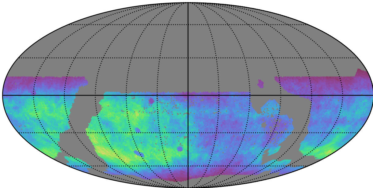
ddf_acor_sf15_lsf20_lsr10_v3.4_10yrs WFD g band: Normalized Teff
