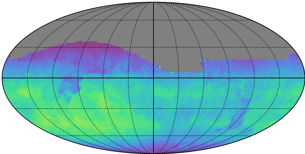
ddf_acor_sf15_lsf20_lsr10_v3.4_10yrs All sky z band: Normalized Teff
