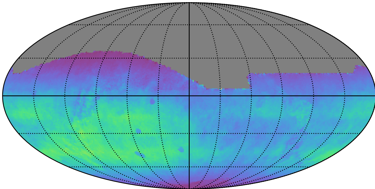
ddf_acor_sf15_lsf20_lsr10_v3.4_10yrs All sky r band: Normalized Teff
