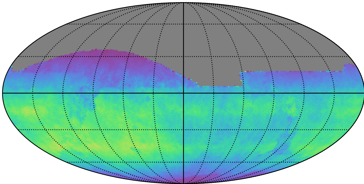
ddf_acor_sf15_lsf20_lsr10_v3.4_10yrs All sky i band: Normalized Teff
